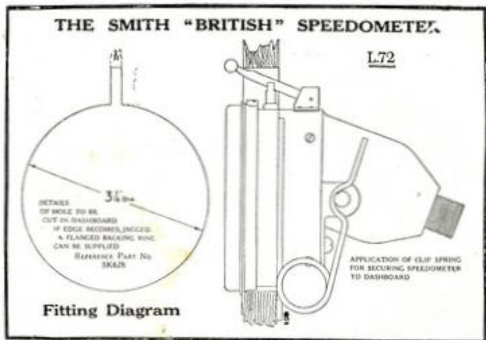
Figure 9. Fitting Diagram. The Smith British Speedometer.
