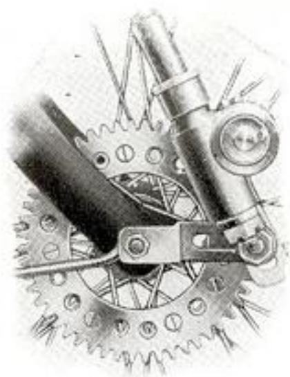
Figure 16. — Type No. AA201. The Smith Motor Cycle Front Wheel Drive.
